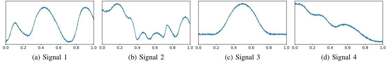
Fig. 3: Noisy synthetic signals
