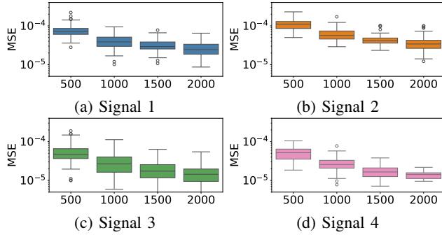
Fig. 5: MSE of SPOP for varying signal lengths
